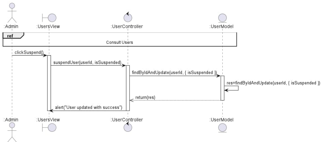
Figure 19: Sequence Diagram – Suspend User
