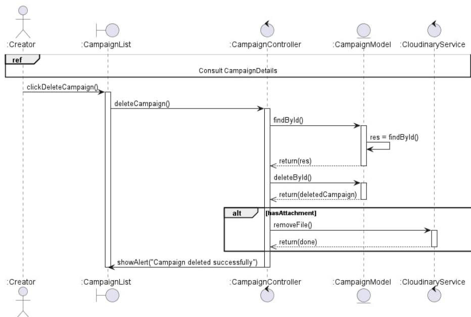
Figure 73: Sequence Diagram – Delete Campaign
