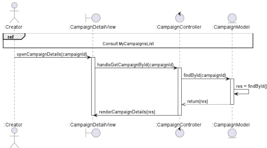
Figure 72: Sequence Diagram – Consult Campaign Details
