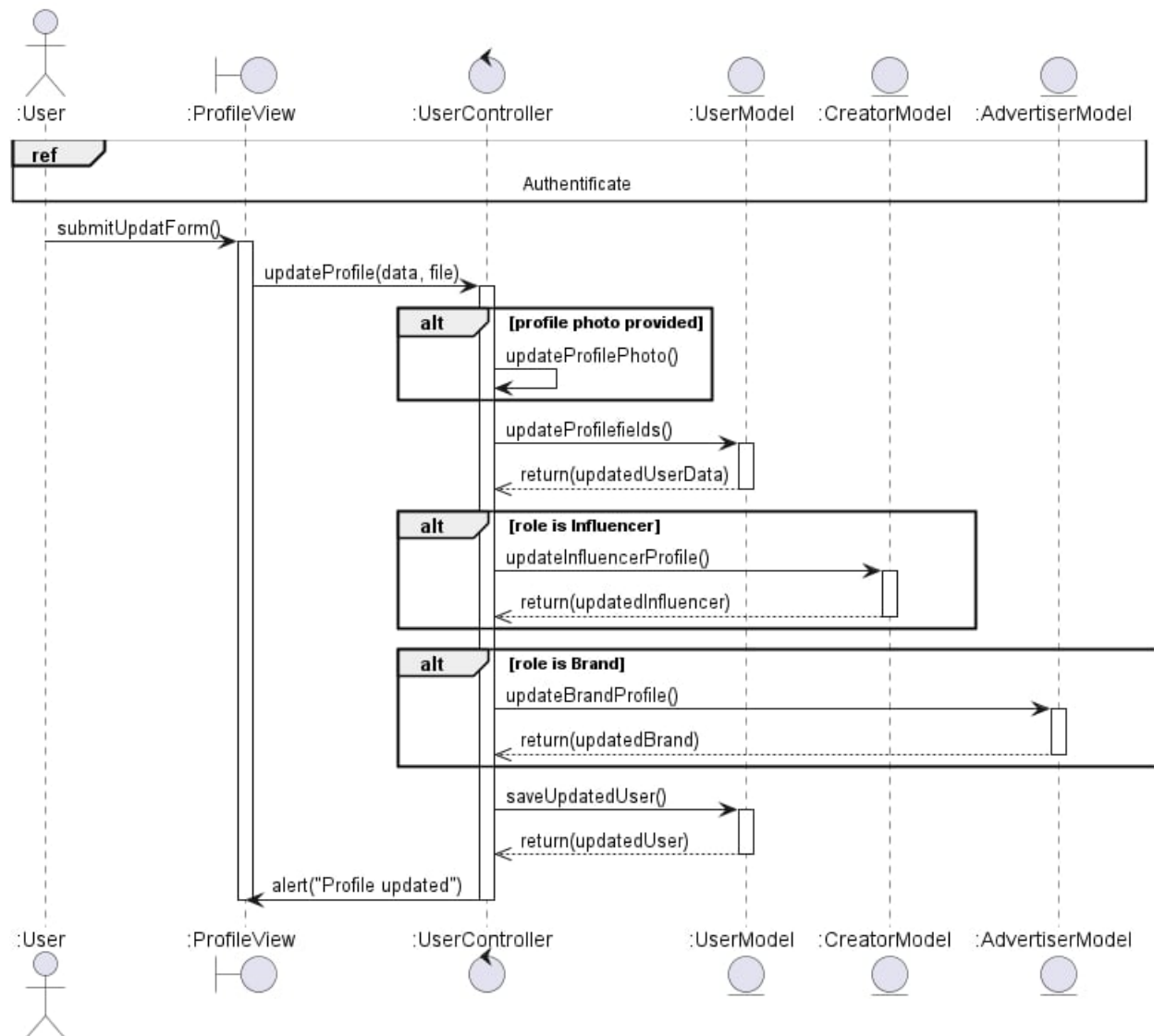
Figure 15: Sequence Diagram – Update Profile
