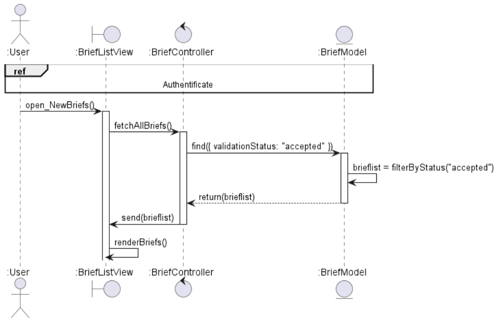
Figure 45: Sequence diagram for consulting list of briefs
