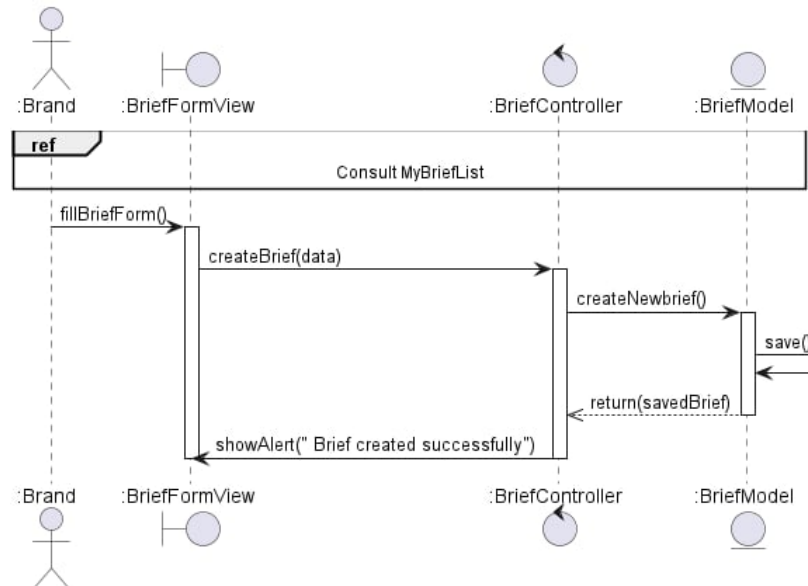
Figure 47: Sequence diagram for creating a new brief
