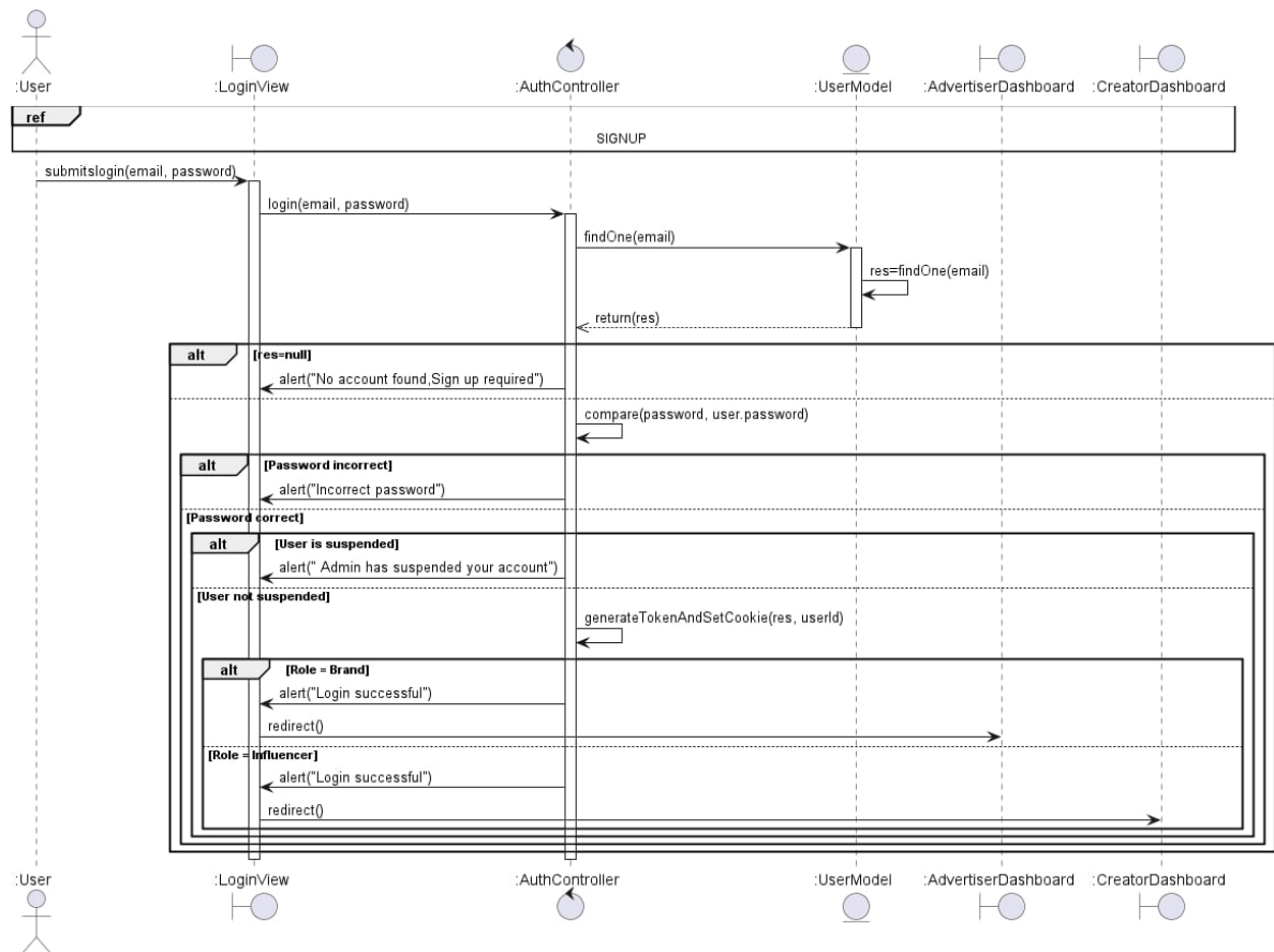
Figure 12: Sequence Diagram – Log In
