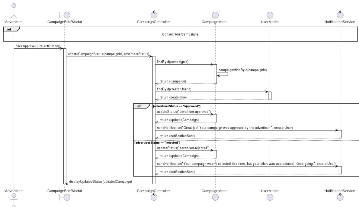
Figure 75: Sequence Diagram – Advertiser Approves or Rejects Campaign
