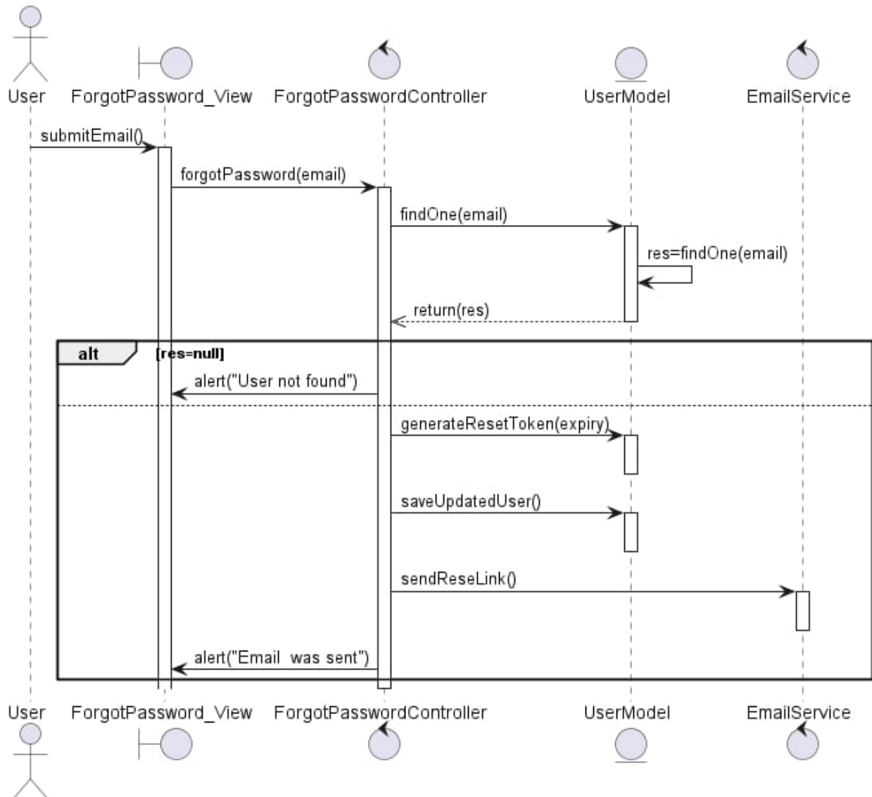
Figure 14: Sequence Diagram – Reset Password
