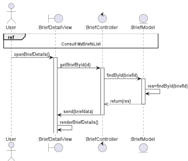
Figure 48: Sequence diagram for consulting brief details
