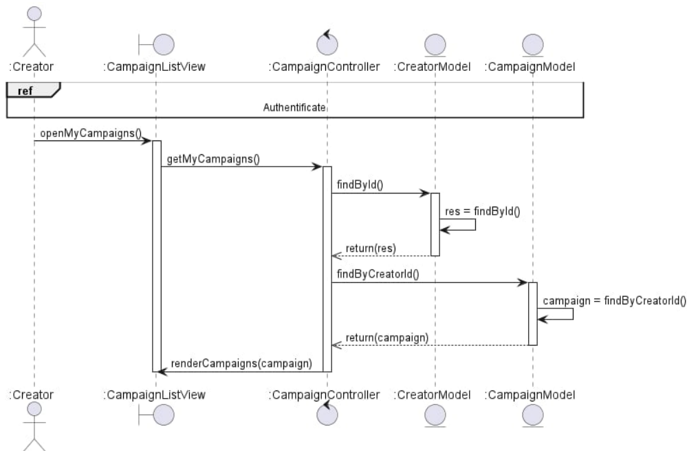
Figure 69: Sequence Diagram – Consult My Campaigns
