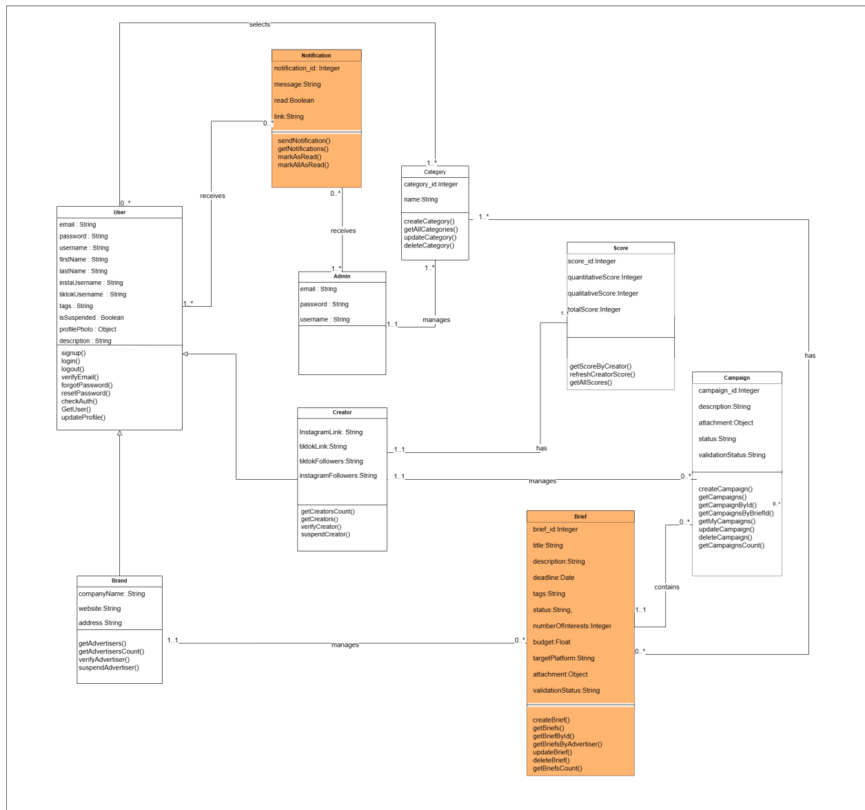
Figure 44: Class Diagram of Sprint 2
