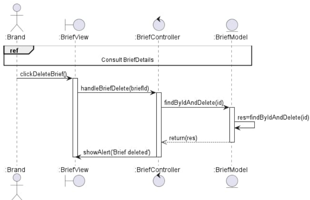
Figure 50: Sequence diagram for deleting a brief
