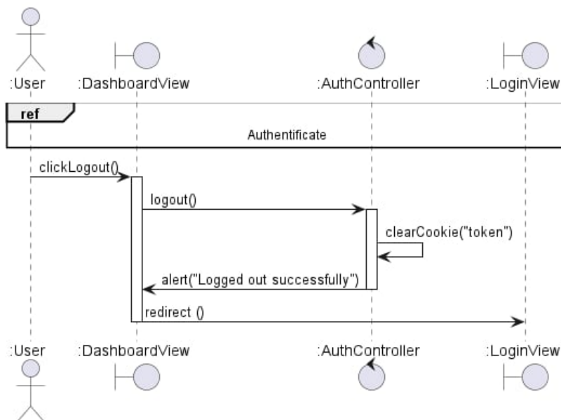
Figure 13: Sequence Diagram – Log Out
