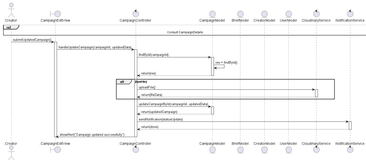
Figure 74: Sequence Diagram – Update Campaign
