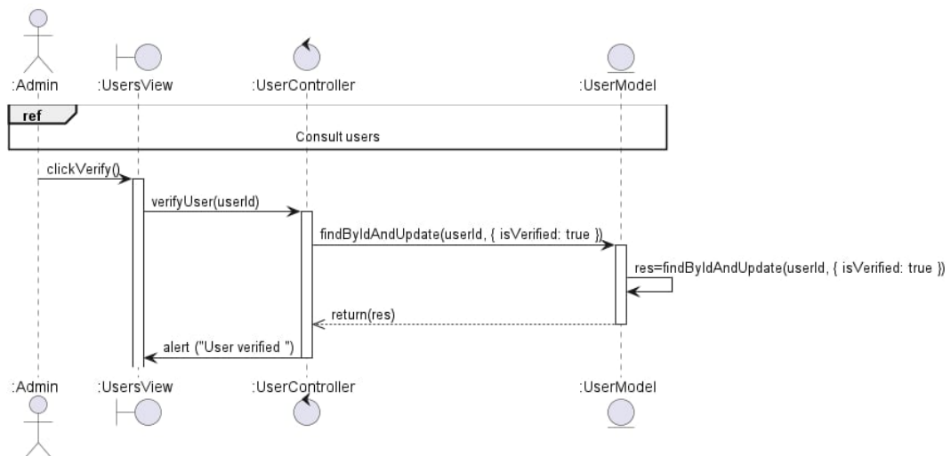
Figure 20: Sequence Diagram – Verify User
