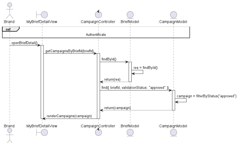
Figure 71: Sequence Diagram – Consult Campaigns Related to a Brief (Brand Perspective)
