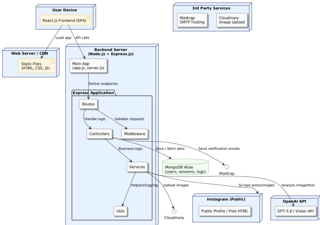
Figure 6: Deployment diagram
