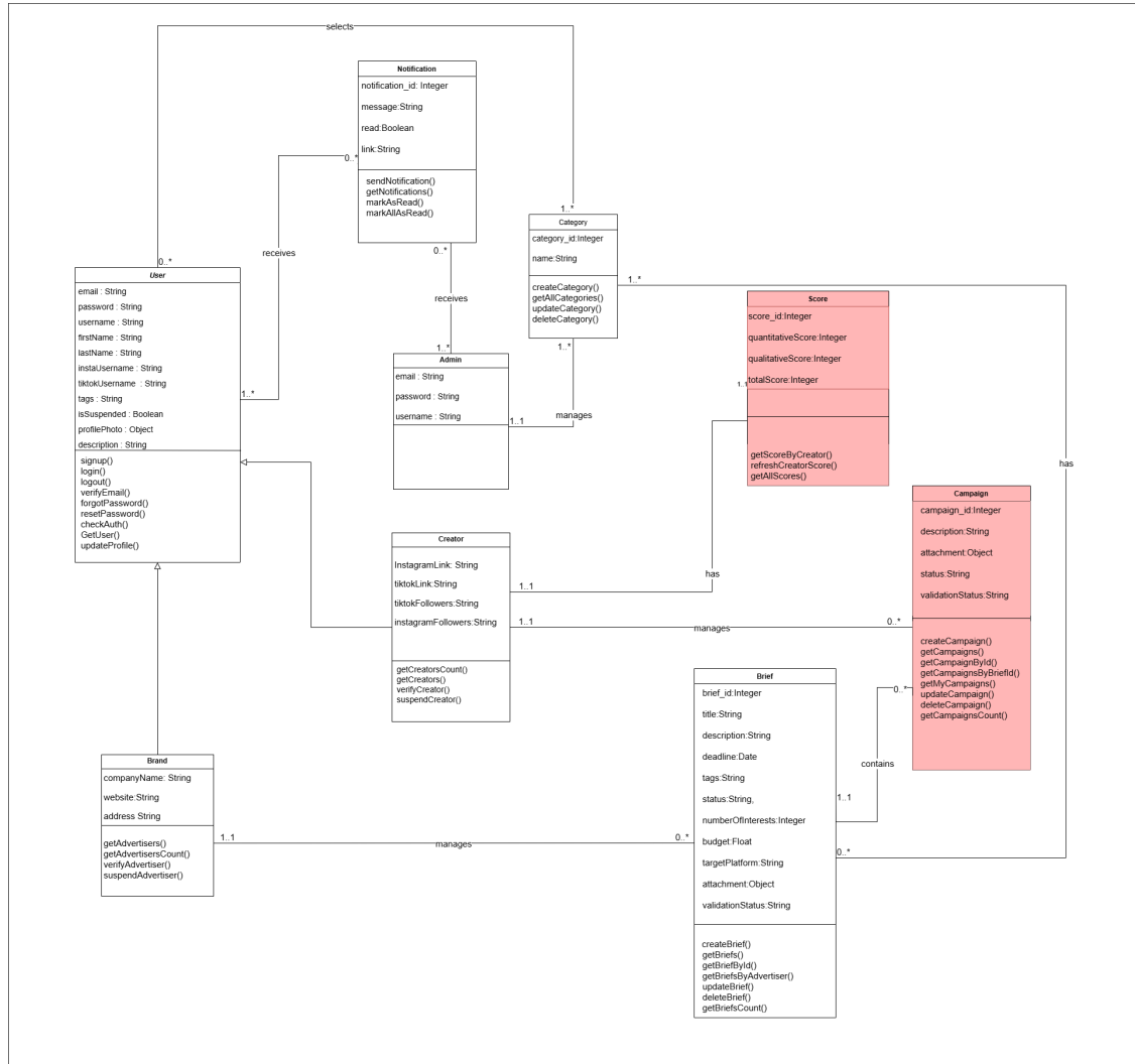
Figure 68: Class Diagram – Sprint 3
