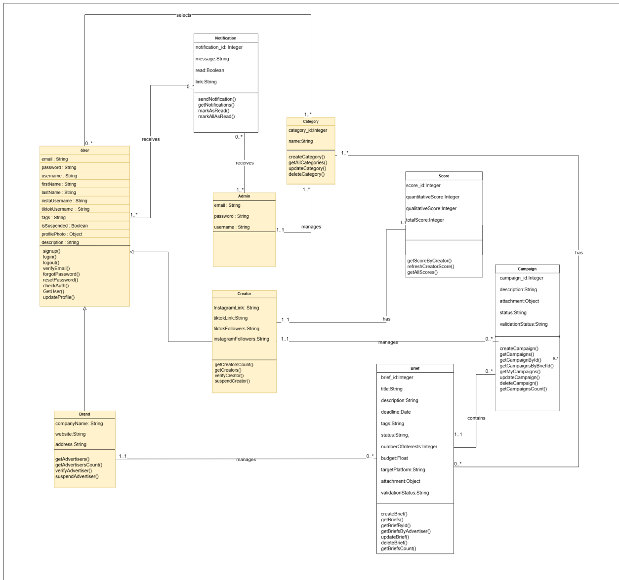
Figure 10: Class Diagram of Sprint 1
