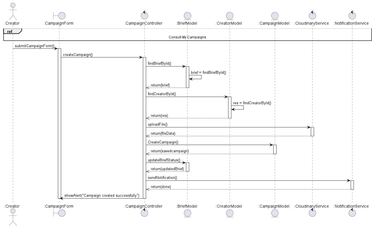
Figure 70: Sequence Diagram – Create Campaign
