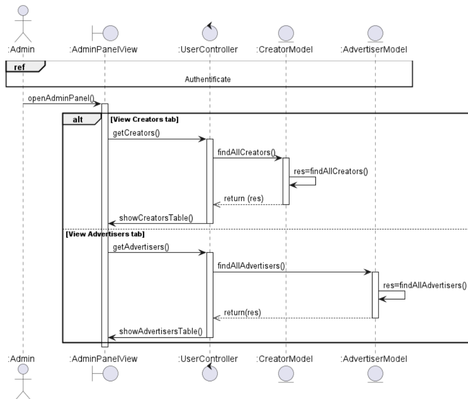
Figure 18: Sequence Diagram – Consult Users
