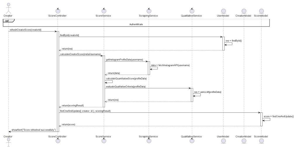
Figure 77: Sequence Diagram – Refresh and Calculate Creator Score
