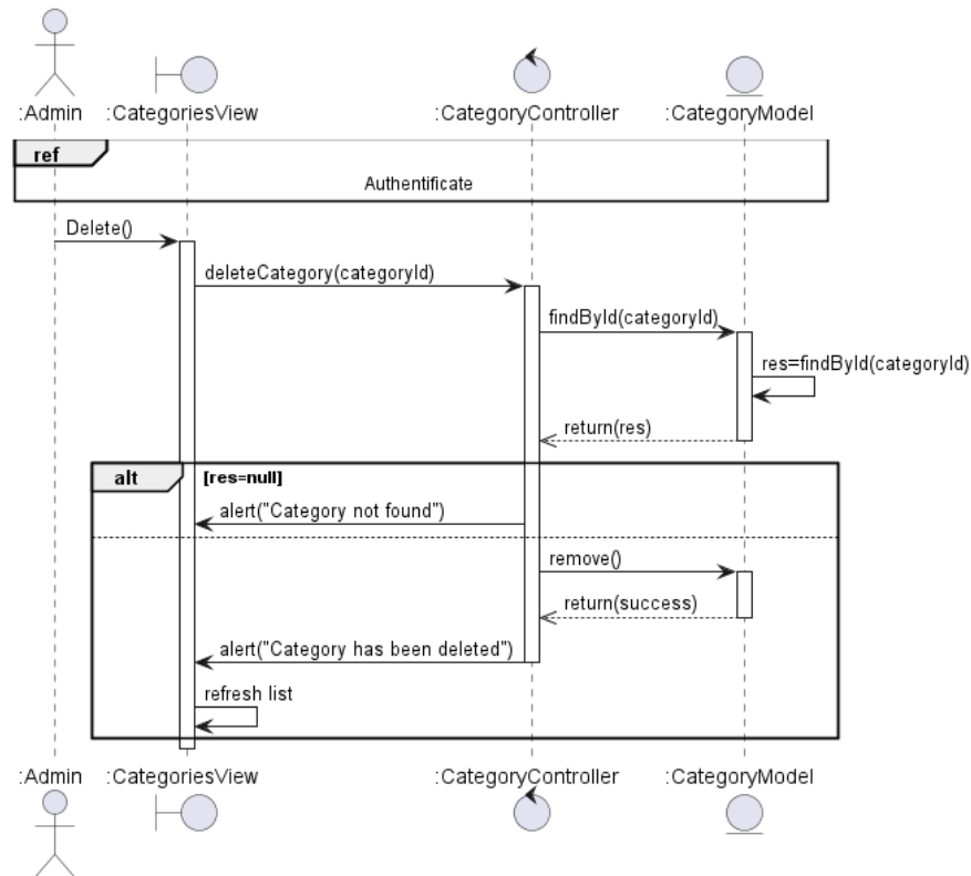
Figure 23: Sequence Diagram – Delete Category
