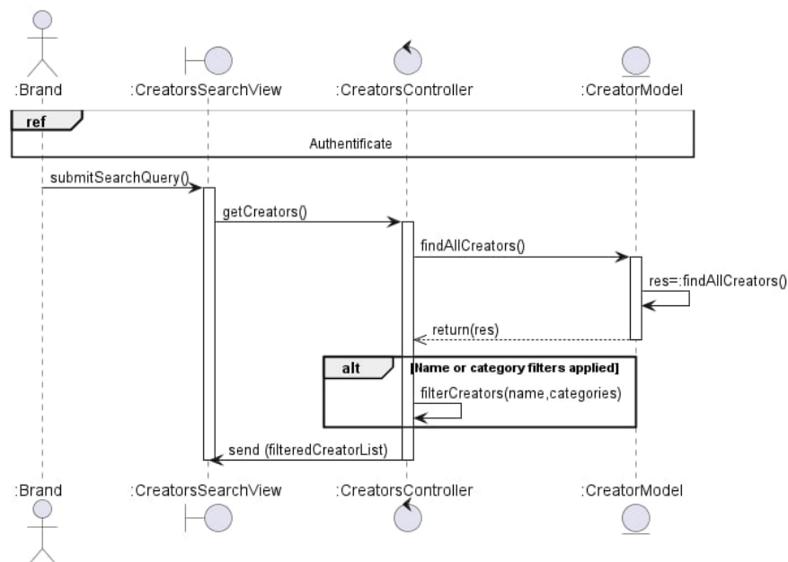
Figure 17: Sequence Diagram – Search Creators
