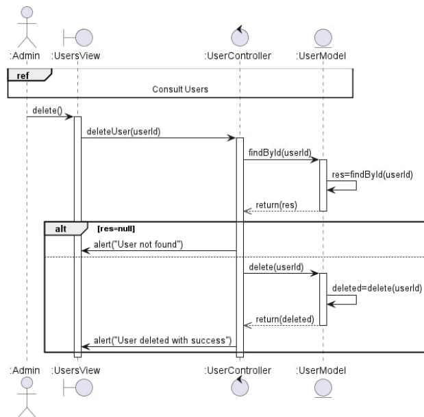
Figure 21: Sequence Diagram – Delete User
