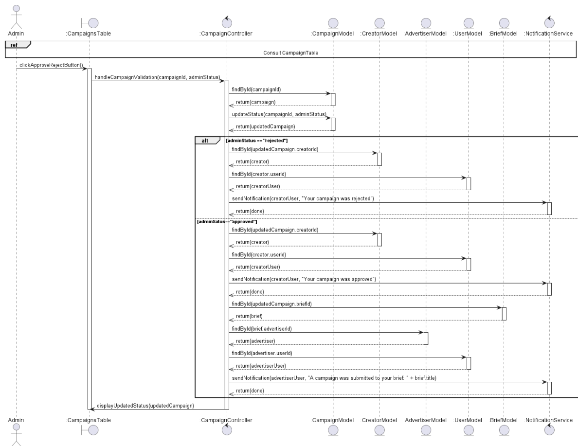
Figure 78: Sequence Diagram – Admin Changes Campaign Status
