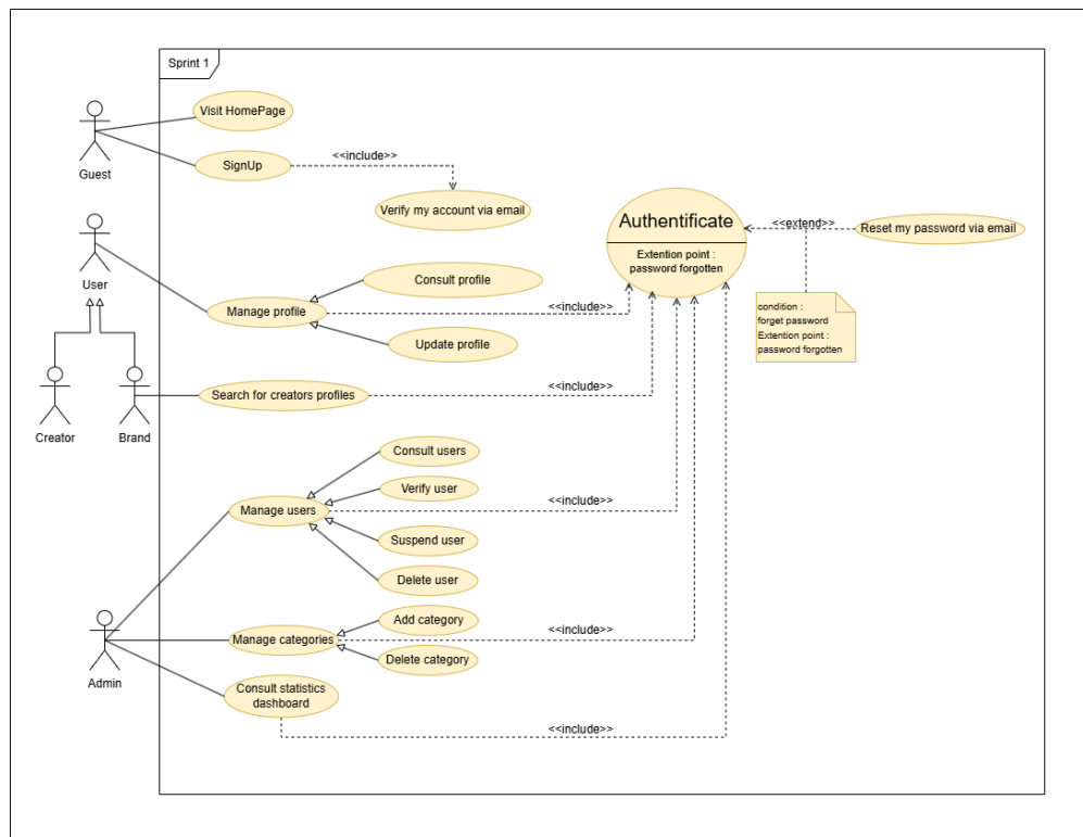
Figure 9: Use Case Diagram – Sprint 1
