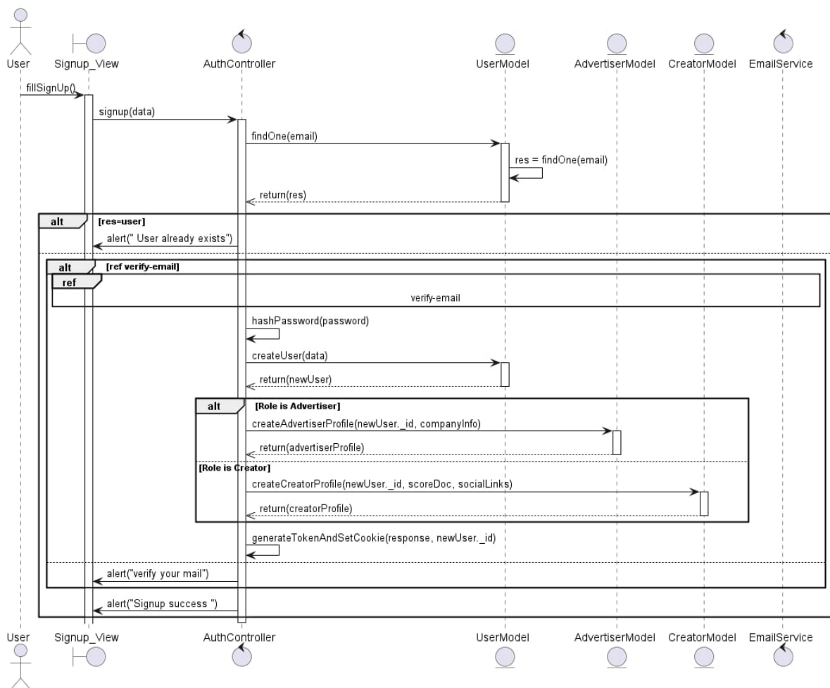
Figure 11: Sequence Diagram – Sign Up
