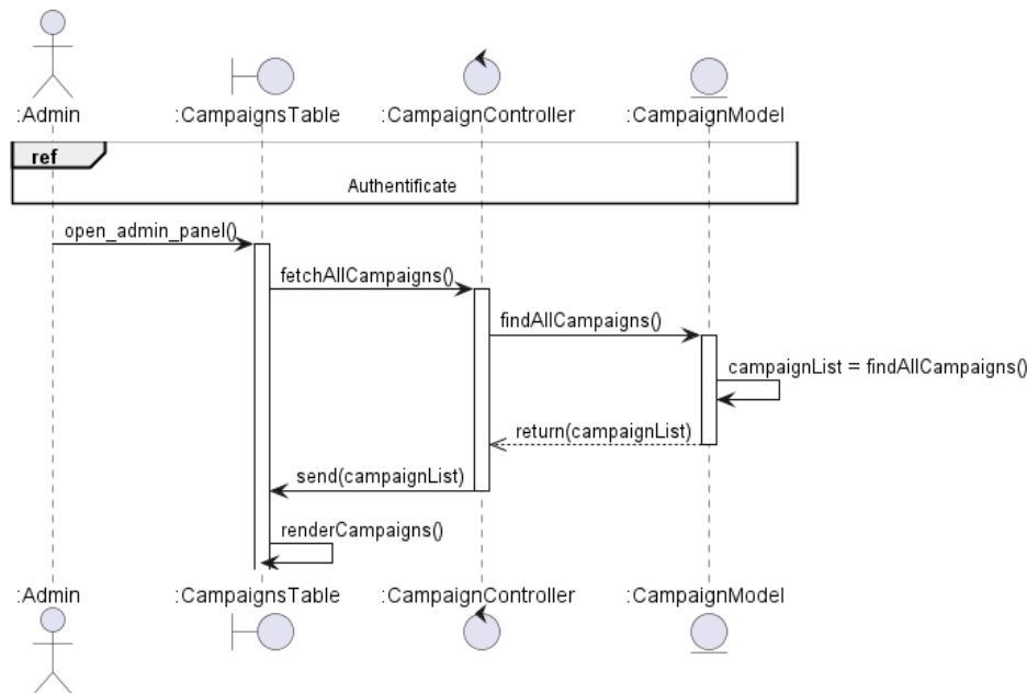
Figure 79: Sequence Diagram – Admin Consults Campaign List
